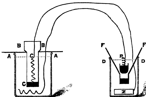
Fig. 251. A A. Outer vessel of the single-pair battery, containing a zinc plate and a solution of common salt. B B. Inverted lamp-glass closed at the bottom with plaster of Paris, and containing a copper plate, c, surrounded with a saturated solution of sulphate of copper. D D. Outer vessel or decomposition cell, containing a weak solution of common salt and amalgamated plate of zinc, z. F F. The funnel closed with plaster of Paris, and holding the little cup of mercury covered and surrounded with a solution of chloride of potassium, P. e. Connecting wire.
